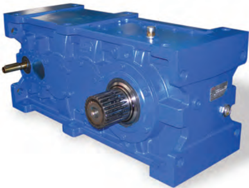
RXP-Parallel Shaft
